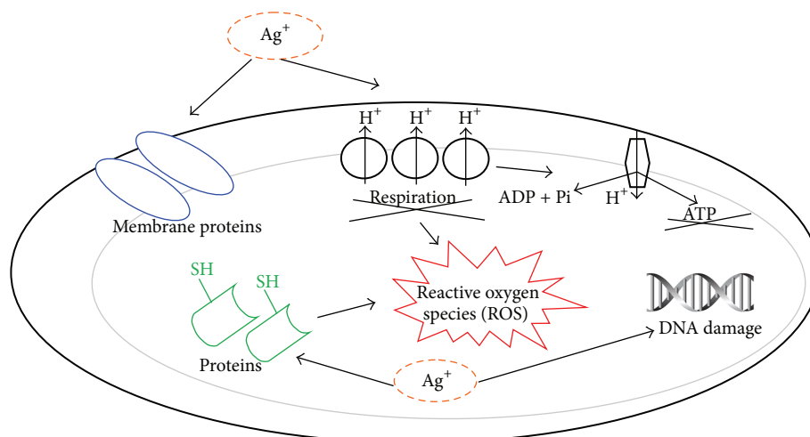
FIGURE 1: Antimicrobial effects of Ag + [33].
